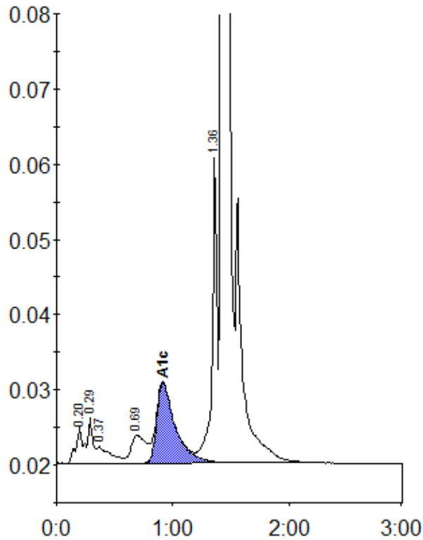
Peak table - ID: 10655060
